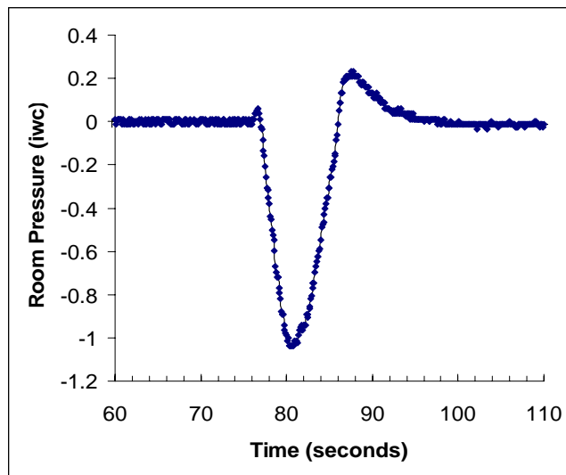
Figure 2. Development of Room Pressure During the Discharge of 6.1% v/v FM-200 ®
